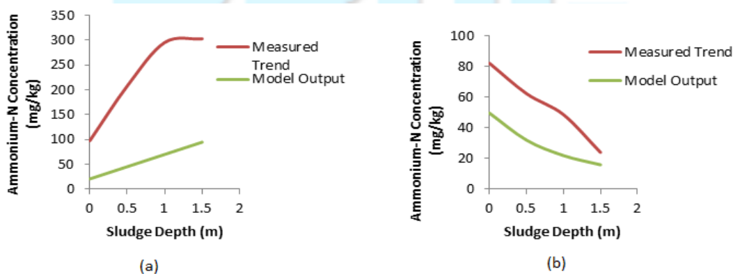
Figure 6: Measured and modeled concentration profiles for ammonium-N in (a) lined pits and (b) unlined pits
