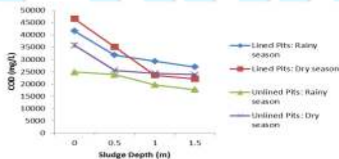
Figure 5: Variation of COD with pit type and season
