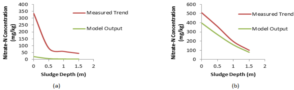
Figure 7: Measured and modeled concentration profiles for nitrate-N in (a) lined pits and (b) unlined pits
