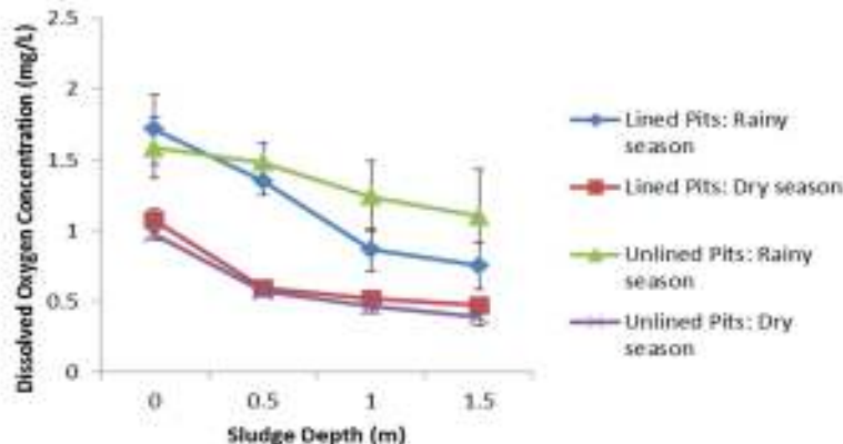
Figure 2: Variation of dissolved oxygen with pit latrine type and season
