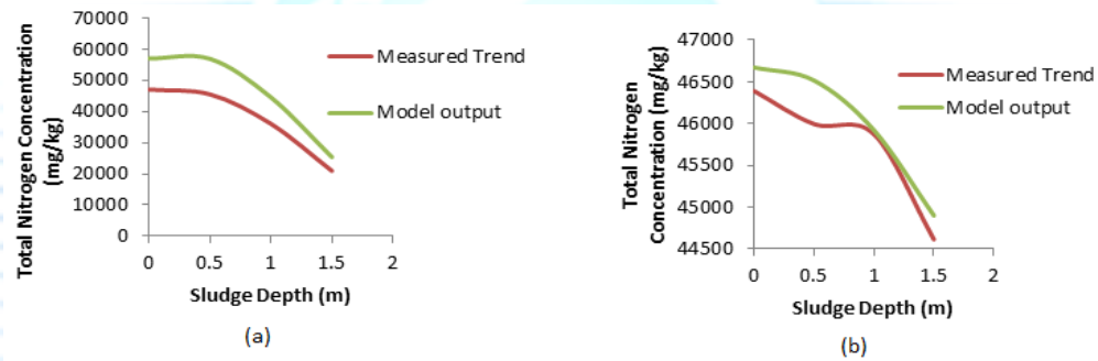
Figure 8: Measured and modeled concentration profiles for total nitrogen in (a) lined pits and (b) unlined pits
