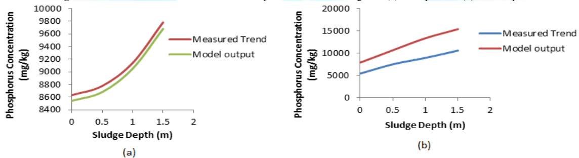
Figure 9: Measured and modeled concentration profiles for phosphorus in (a) lined pits and (b) unlined pits
