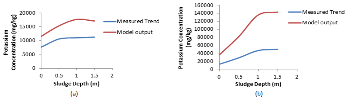
Figure 10: Measured and modeled concentration profiles for potassium in (a) lined pits and (b) unlined pits
