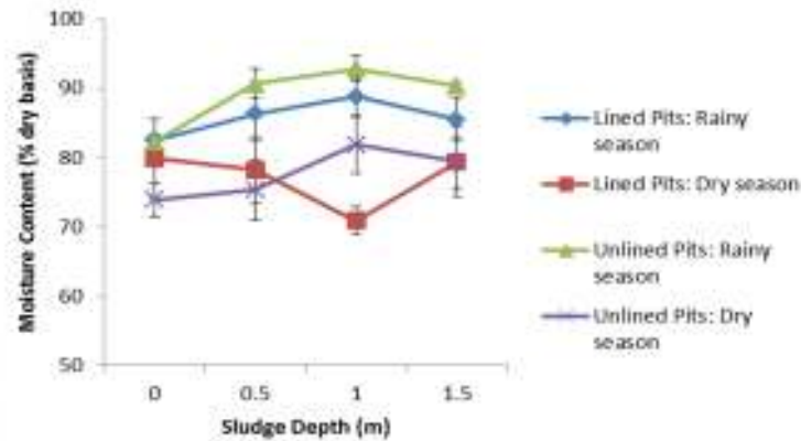
Figure 4: Variation of moisture content with pit type and season
